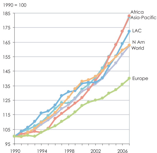
Index of change in GDP, world regions, 1990-2007
