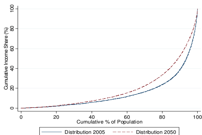
Figure 6.1 Lorenz Dominance: Changes in the middle of the distribution
